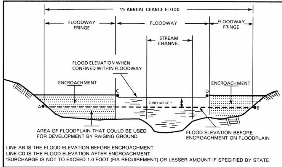
FIGURE 1 – Floodway Schematic
